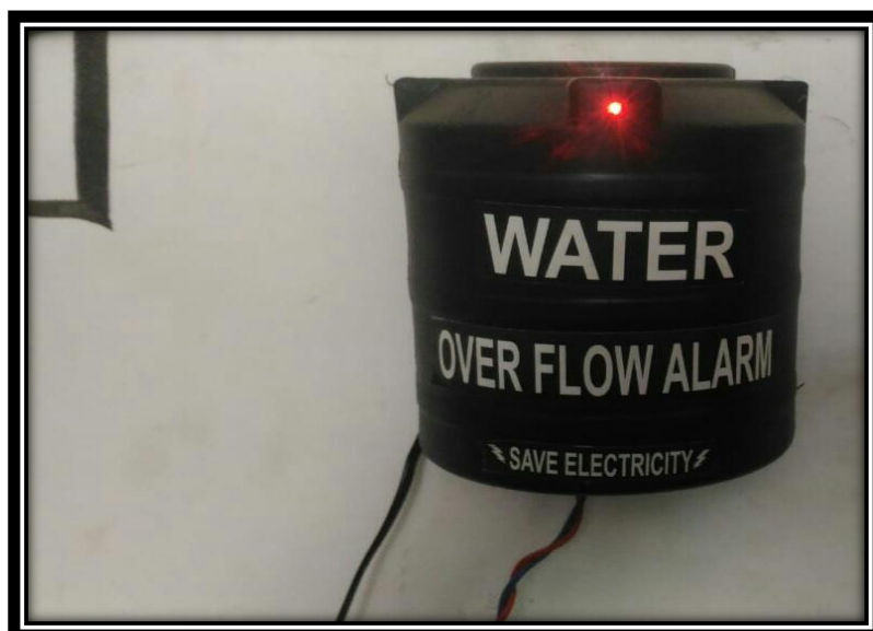
Save water & Save Electricity Alarm
